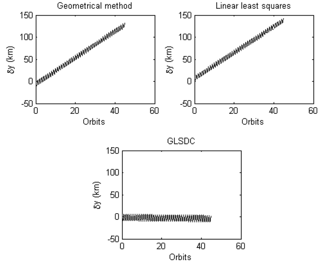
Fig. 8 Error growth comparisons in the in-track direction.
