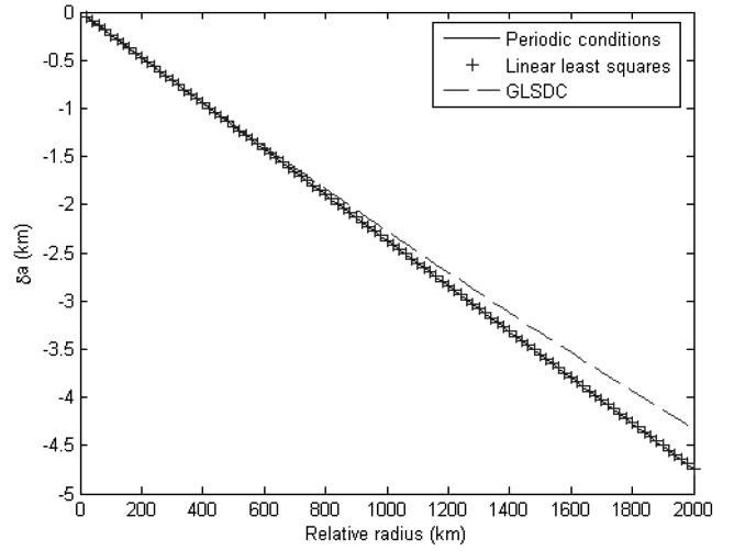
Fig. 7 Comparison for periodic matching conditions.
