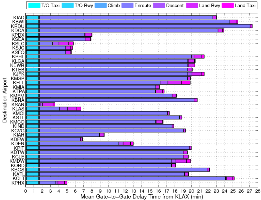
Figure 21. Mean Gate-to-Gate Delays using QNA Analysis with Uncertainties
