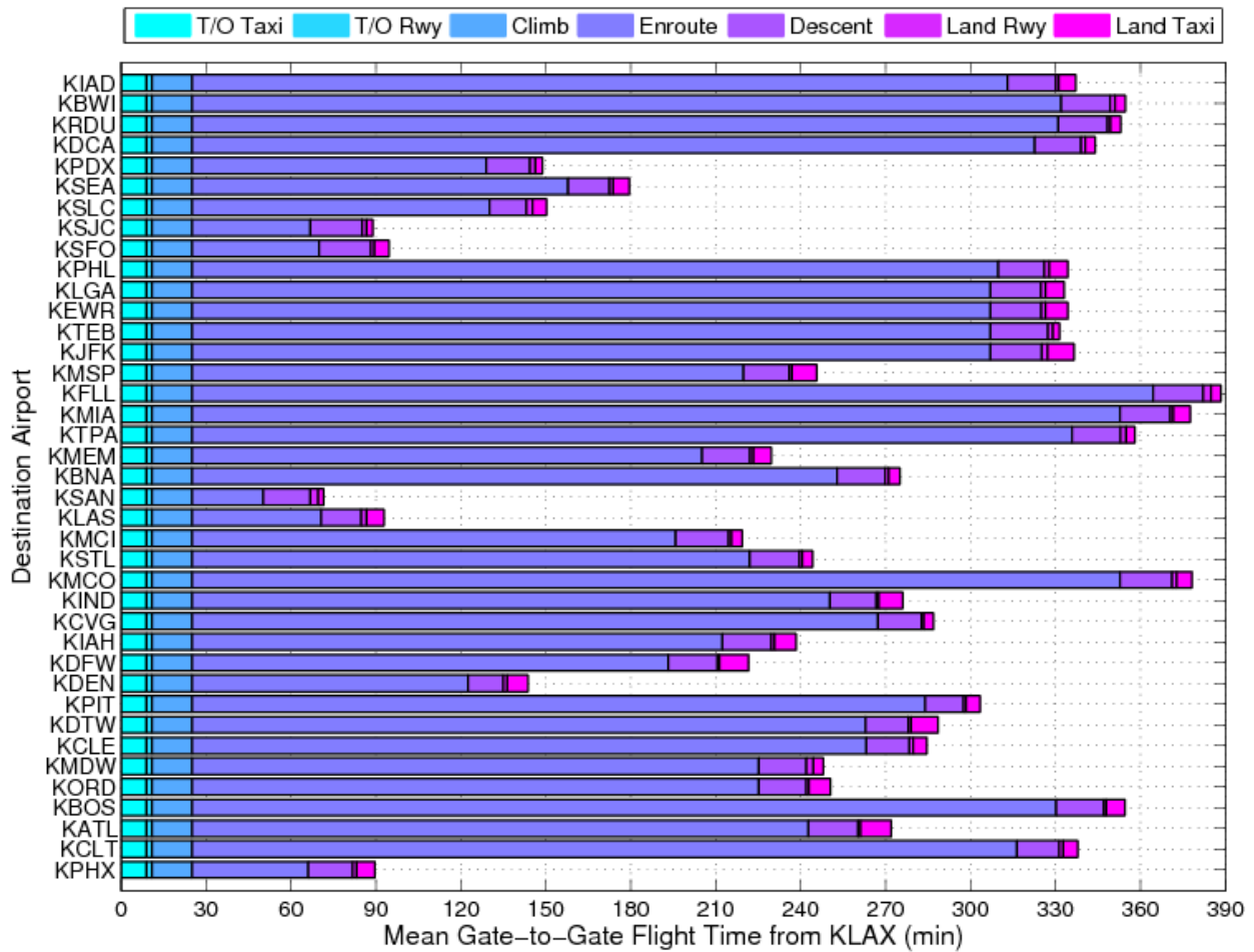
Figure 17. Mean Gate-to-Gate System Times using QNA Analysis with Nominal Data
